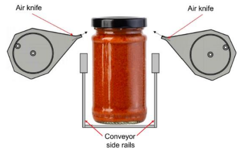
Figure 5: Blower System knife setup
