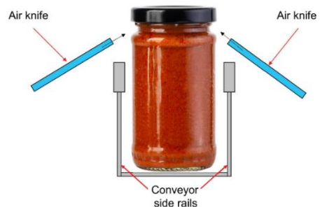
Figure 6: Forced Air knife setup
