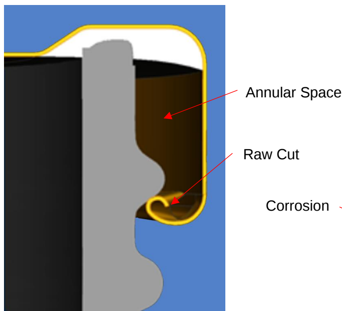
Figure 1: Fully applied steel closure sectioned view of the curl
