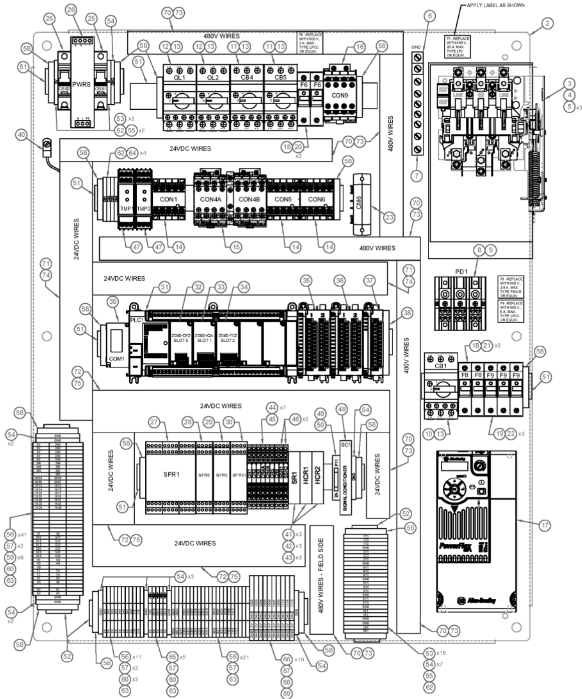
CONTROL PANEL AND OTHER ASSEMBLED COMPONENTS WIRING SPECIFICATIONS
